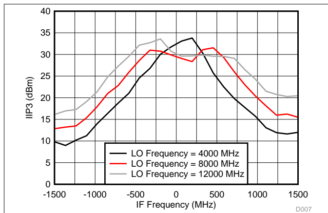
图 9. IIP3 Across IF Frequency for Internal LO Mode
