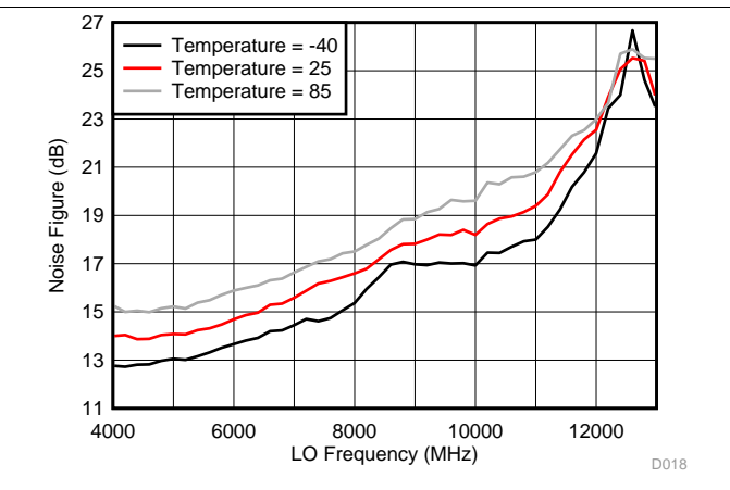
图 20. Noise Figure Across LO Frequency for External LO Mode
