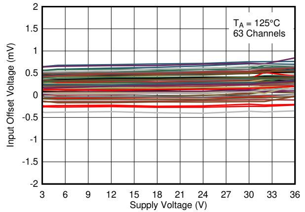
Figure 6-17. Input Offset Voltage vs. Supply Voltage at 125^\circ\text{C}
