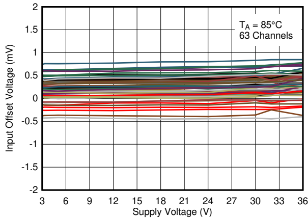
Figure 6-16. Input Offset Voltage vs. Supply Voltage at 85^\circ\text{C}
