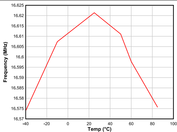
Figure 7-14. High Frequency Oscillator (HFO) Accuracy vs. Temperature
