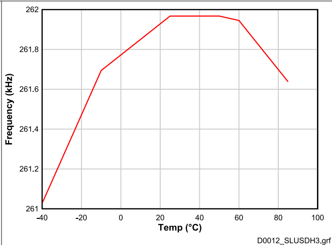
LFO measured in FULL SPEED mode (262 kHz) Figure 7-13. Low Frequency Oscillator (LFO) Accuracy vs. Temperature
