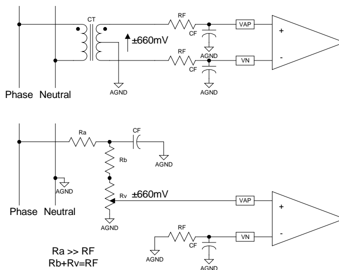
Figure 5. Typical Connections for Voltage Channels
