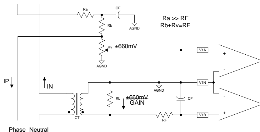
Figure 7. Typical Connections for Current Channels
