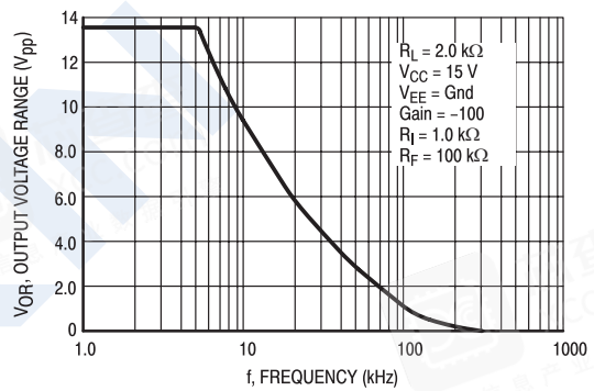
Figure 4. Large-Signal Frequency Response
